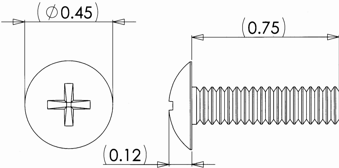
10X32 UNC Standard Rack Screw
