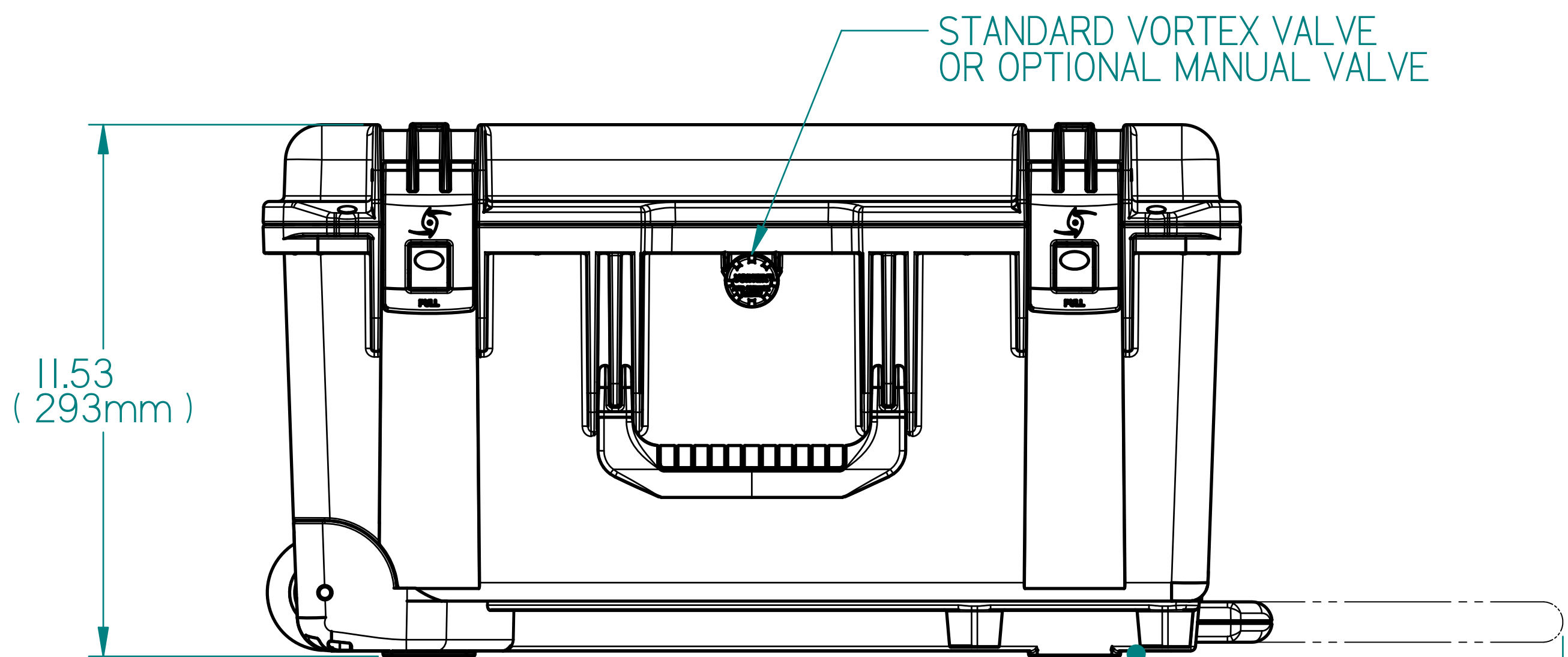
FRONT VIEW
