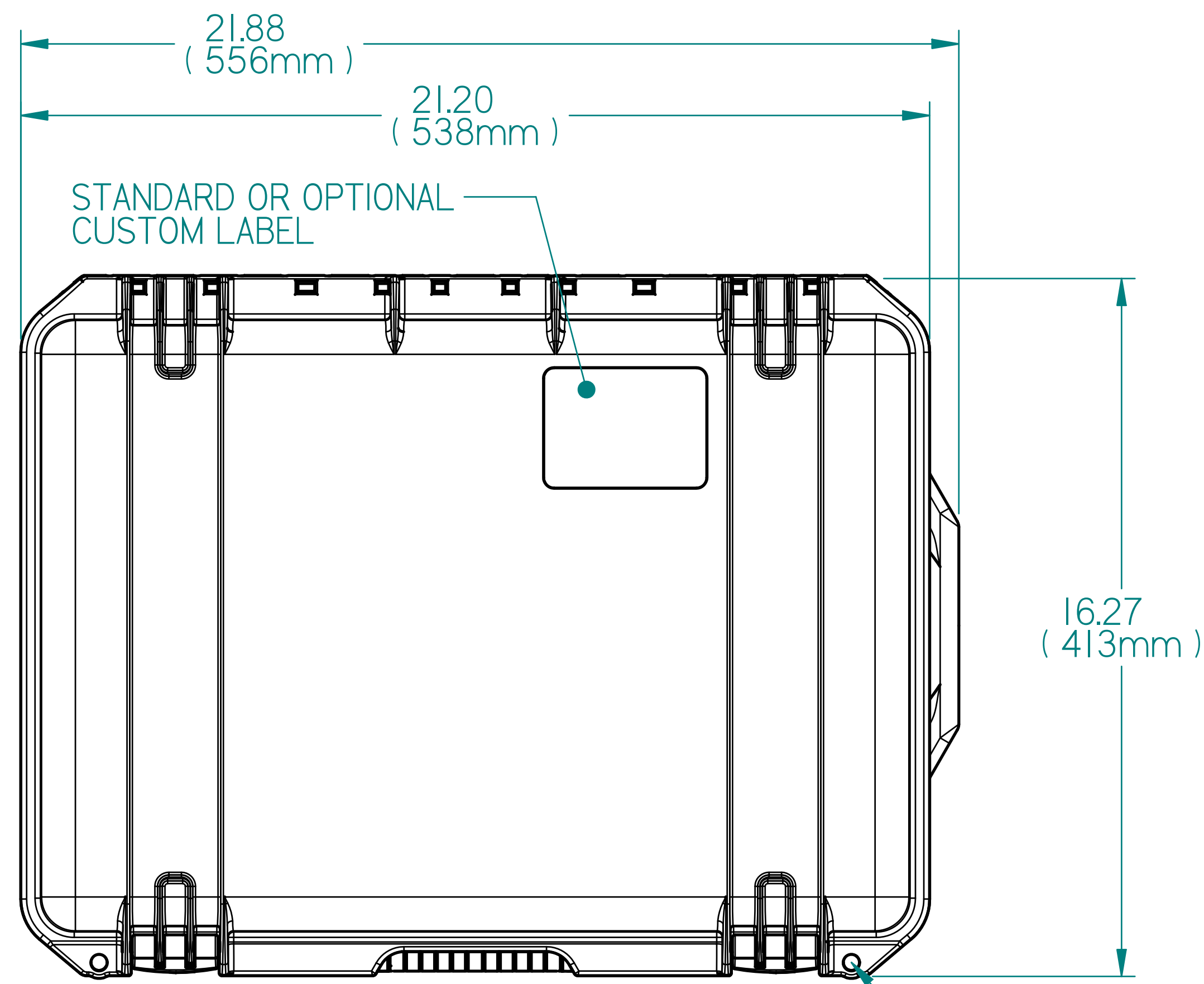
TOP VIEW
